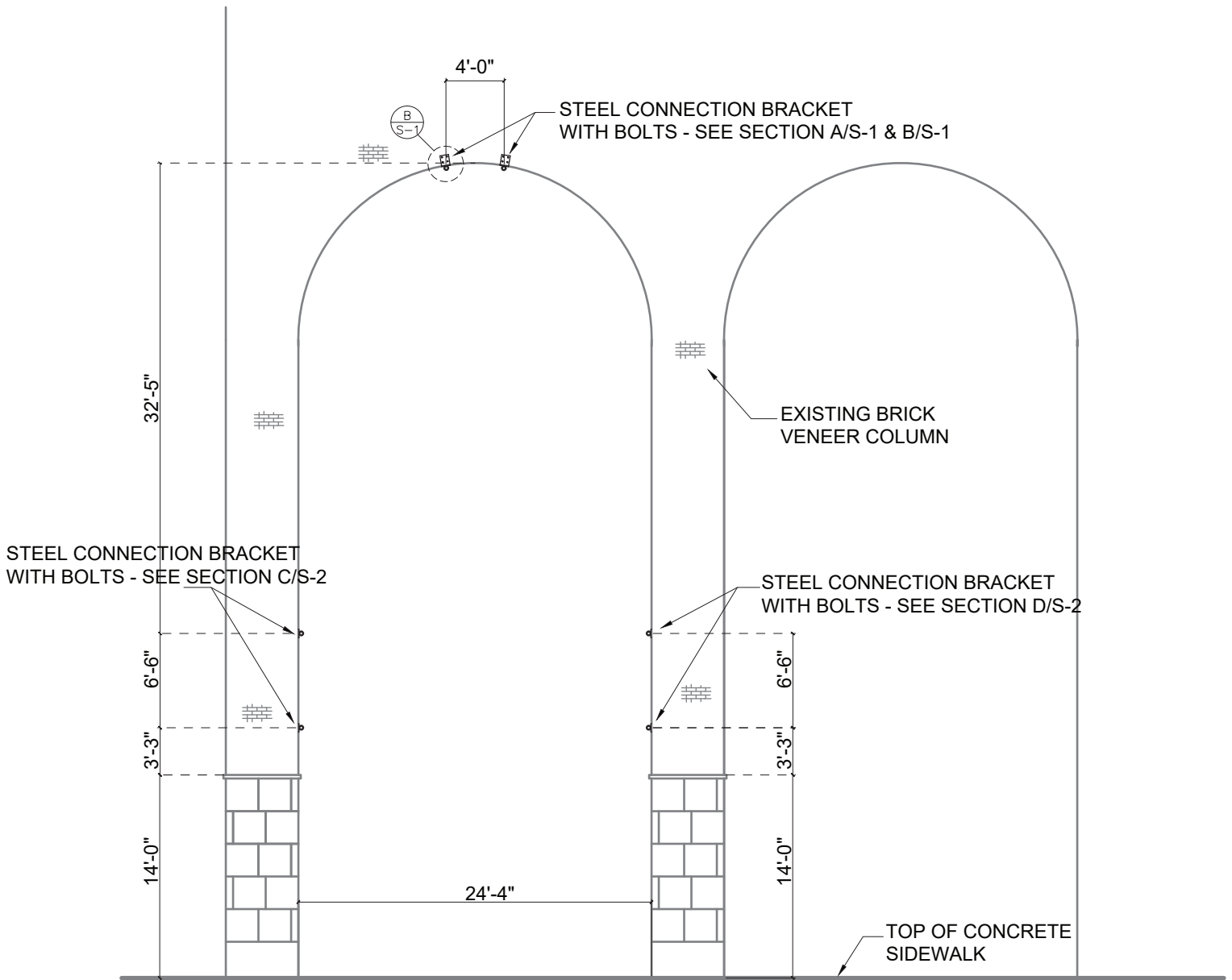
SOUTH ELEVATION of EXTERIOR ARCHWAY
